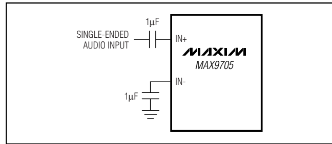
Figure 5. Single-Ended Input
